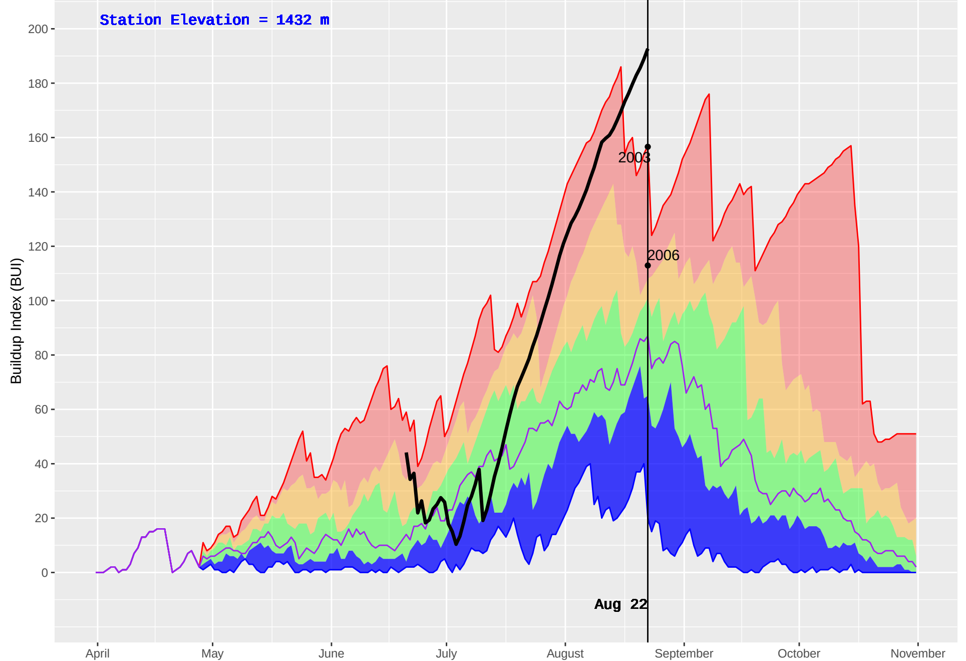
OCTOPUS CREEK (396) : Historical (2000–2016) and Current (2018) Daily Buildup Index (BUI)
