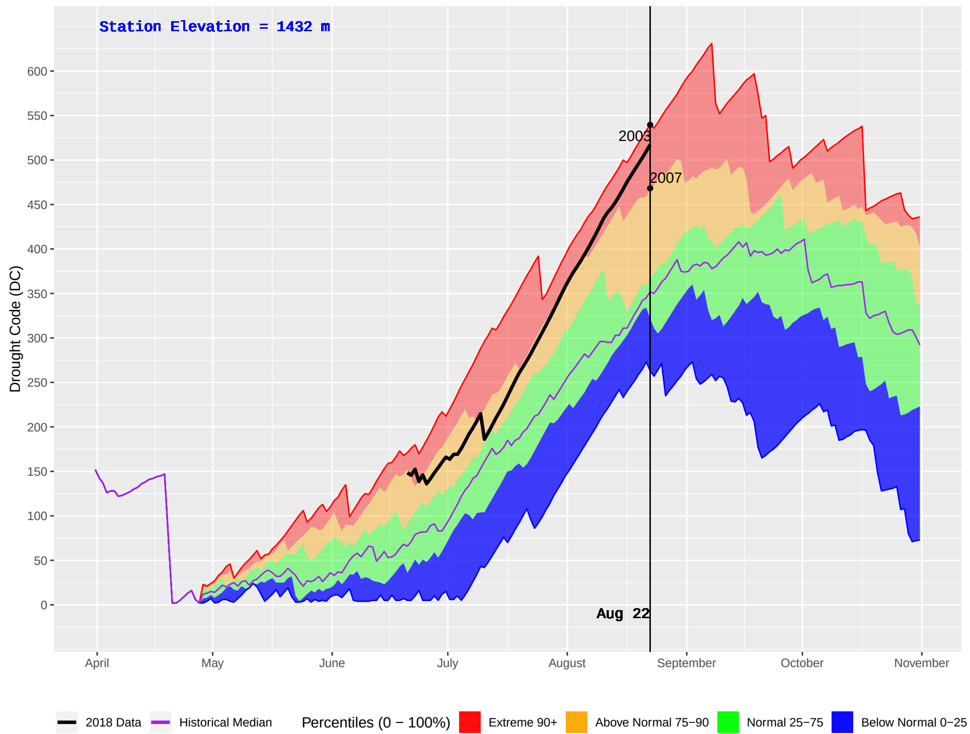
OCTOPUS CREEK (396) : Historical (2000–2016) and Current (2018) Daily Drought Code (DC)
