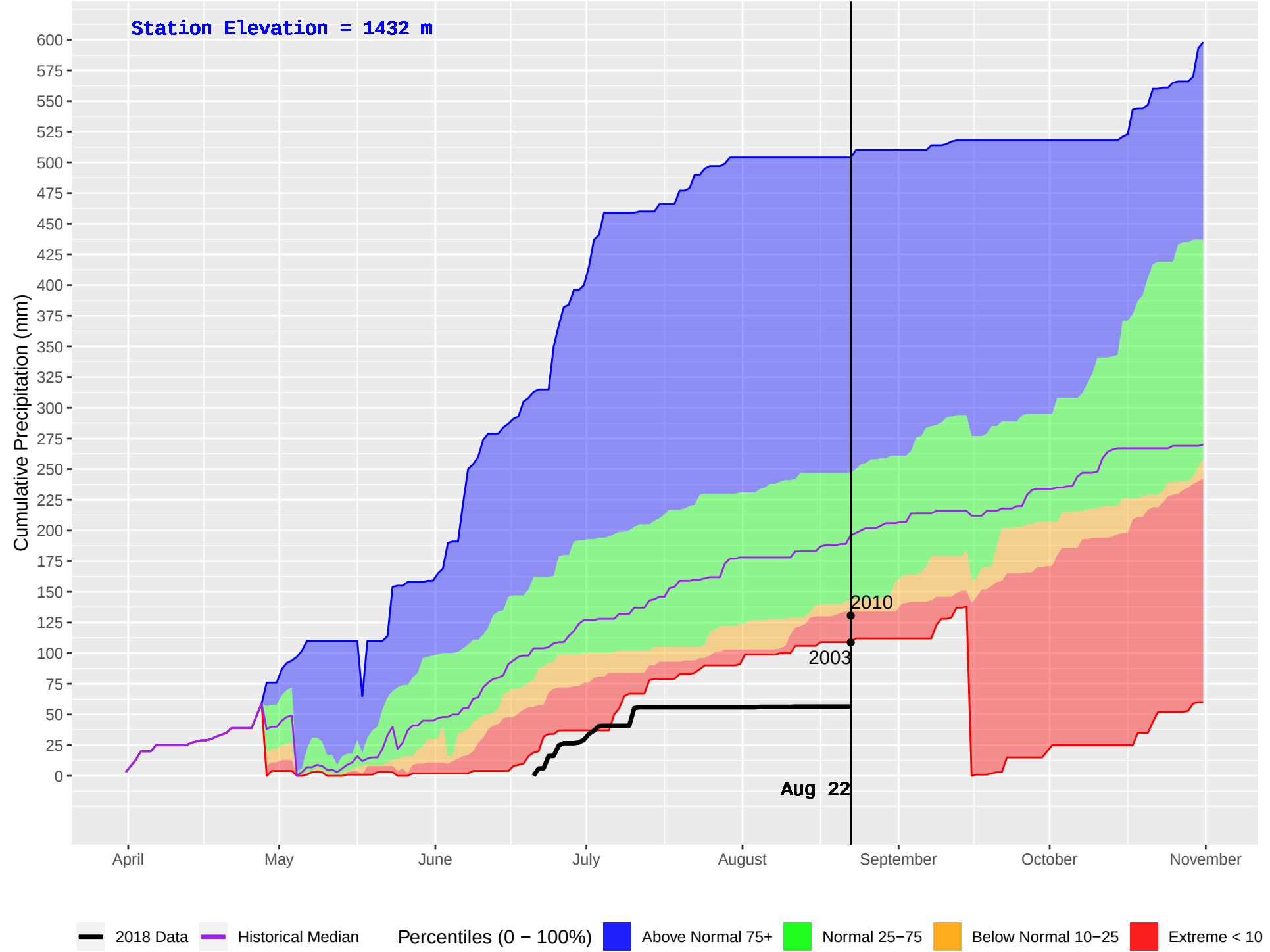
OCTOPUS CREEK (396) : Historical (2000–2016) and Current (2018) Daily Cumulative Precipitation
