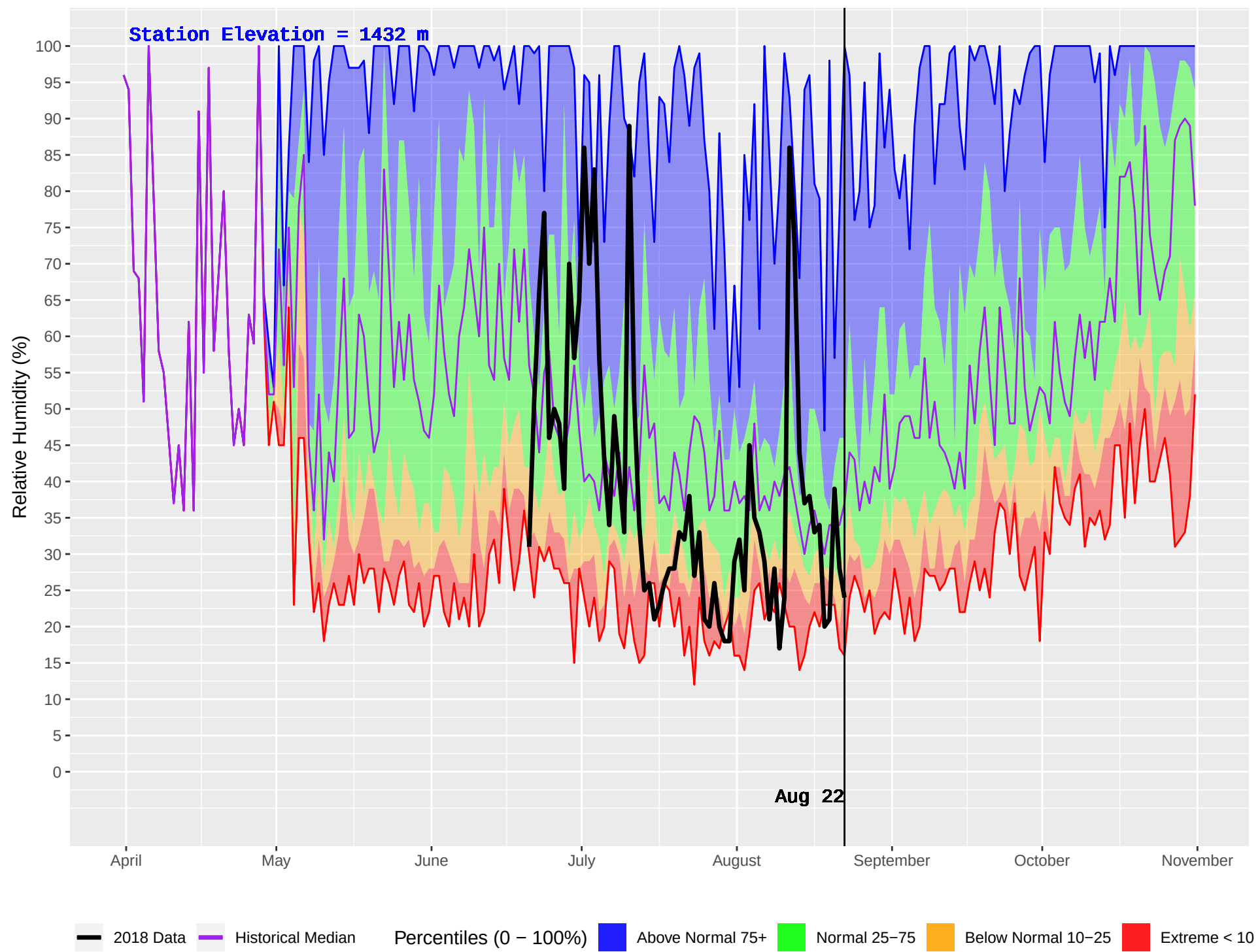
OCTOPUS CREEK (396) : Historical (2000–2016) and Current (2018) Daily Relative Humidity
