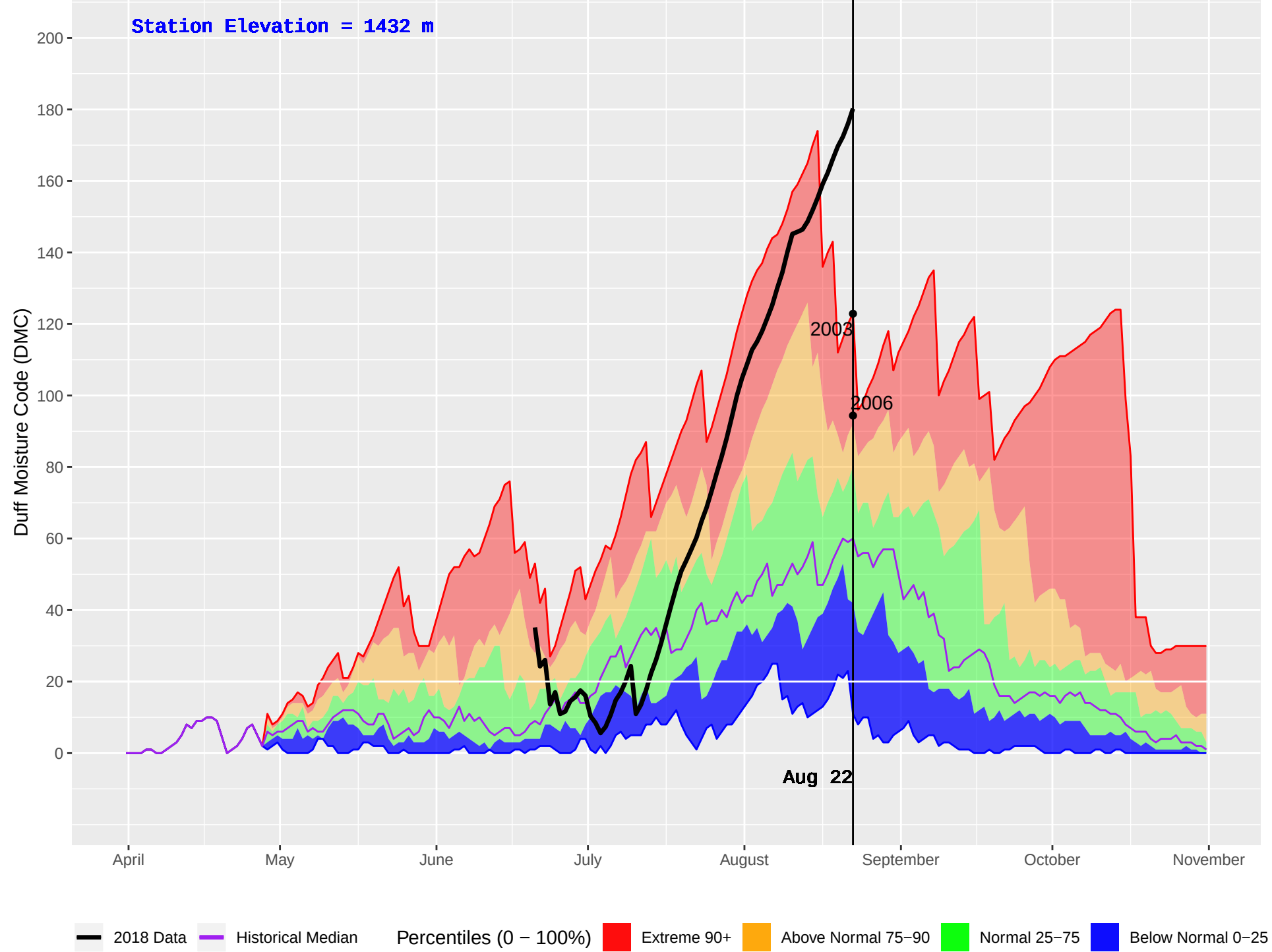
OCTOPUS CREEK (396) : Historical (2000–2016) and Current (2018) Daily Duff Moisture Code (DMC)
