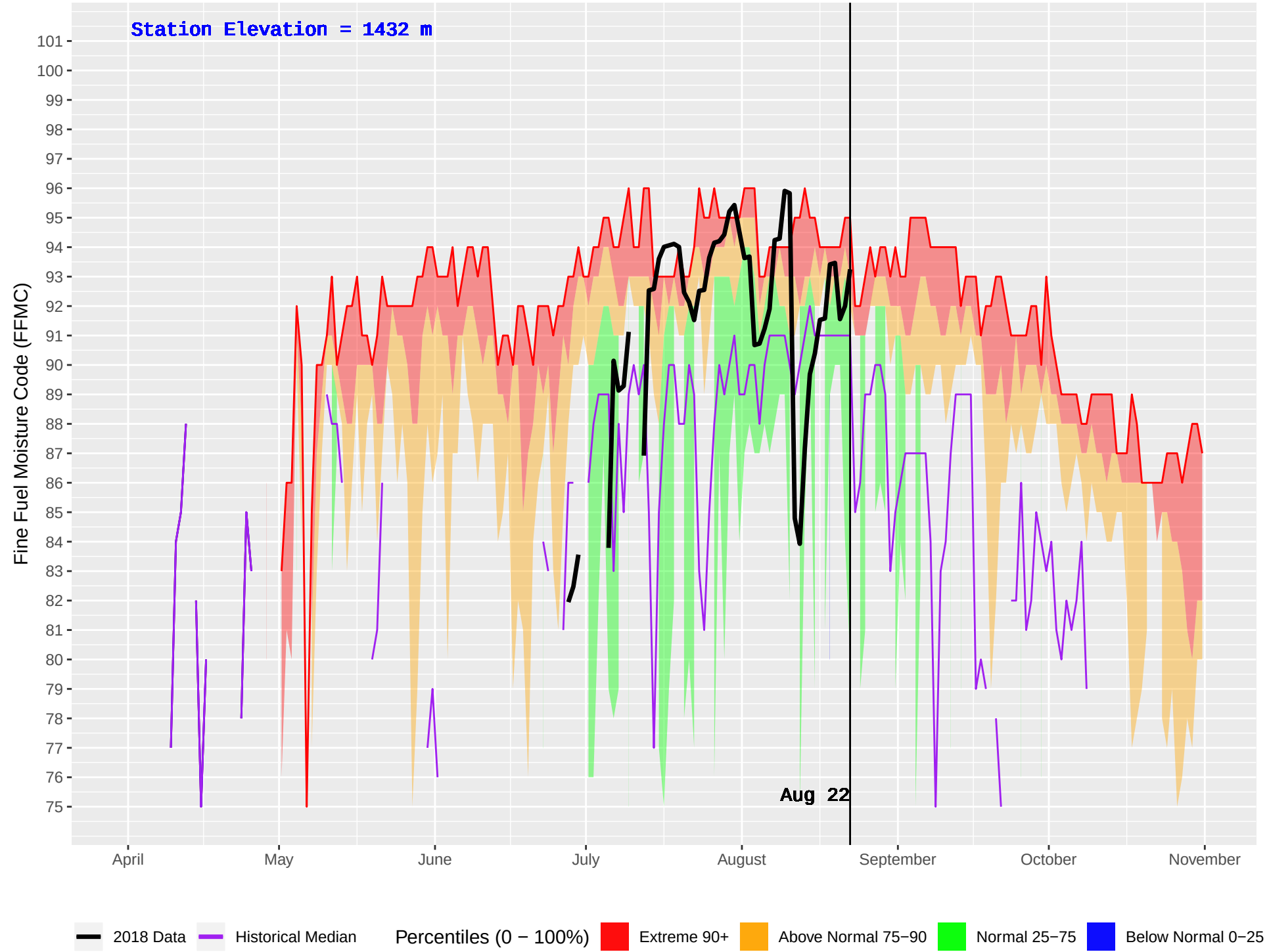
OCTOPUS CREEK (396) : Historical (2000–2016) and Current (2018) Daily Fine Fuel Moisture Code (FFMC)
